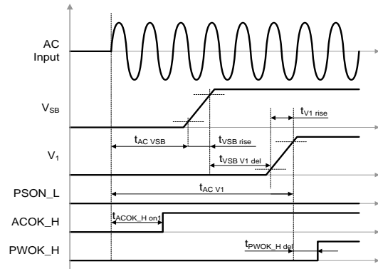
Figure 25. AC turn-on timing
