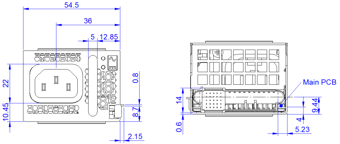
Figure 44. Front and Rear View
